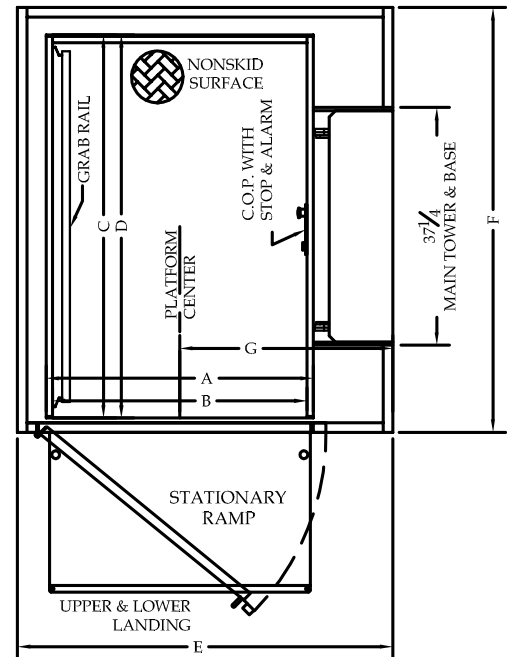
LOWER LANDING STATIONARY RAMP APPLICATION SHOWN
